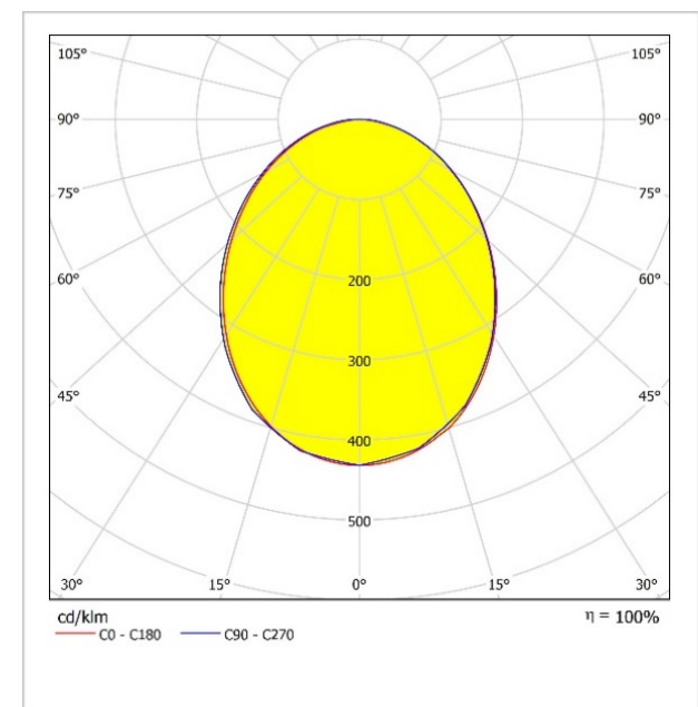
Photometric Curve
