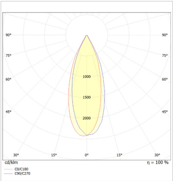
Photometric Curve
