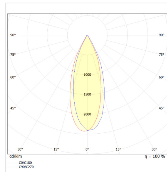
Photometric Curve
