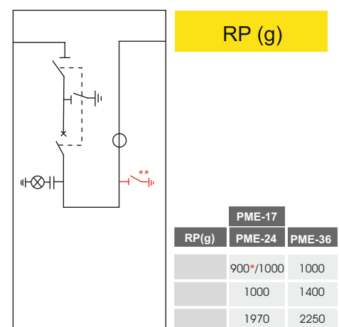
Cubicle Connection Cubicle with Circuit Breaker (with SF6 Insulated Disconnector)
