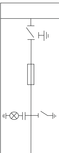
Cubicle with Fused Disconnector (with Air Rotary Disconnector) * for PME-24
