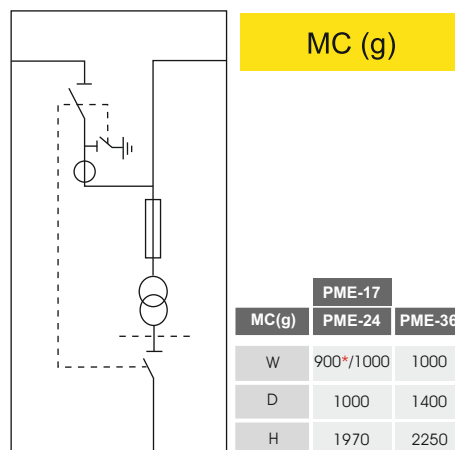
Current Voltage Measurement Cubicle (with SF6 Insulated Disconnector)
