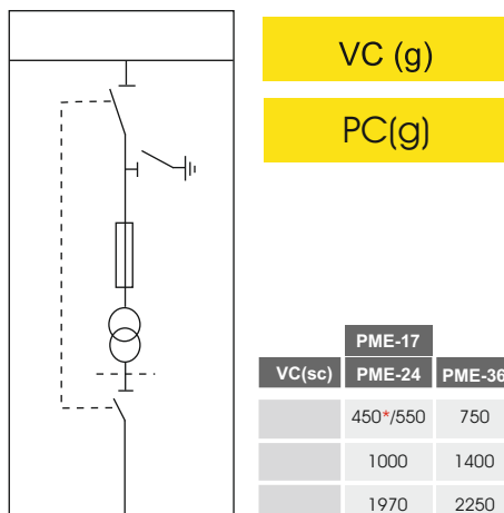
Voltage Measurement Cubicle (with SF6 Insulated Disconnector)
