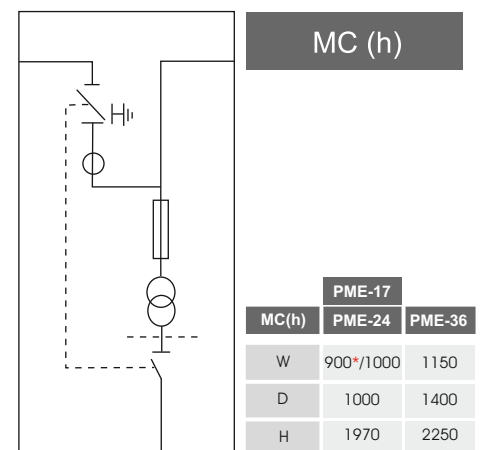
Current Voltage Measurement Cubicle (with Air Rotary Disconnector)
