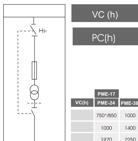
Voltage Measurement Cubicle (with Air Rotary Disconnector)
