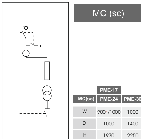
Current Voltage Measurement Cubicle (with Switch Disconnector)
