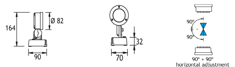
horizontal adjustment
