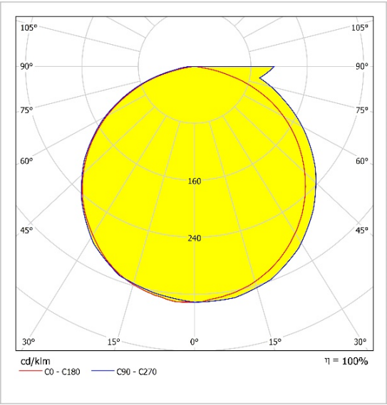
Photometric Curve
